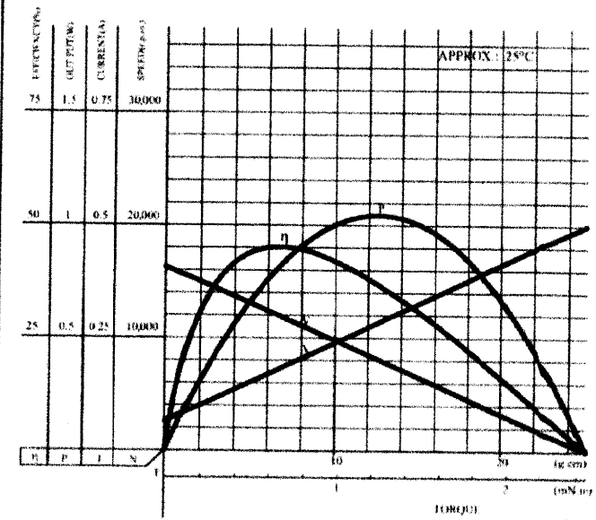
Motor Performance Curve
